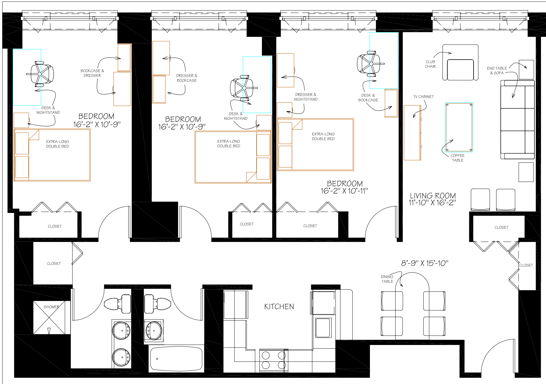
TYPE 9 Typical Apartment - 3 Bedroom - 1280 sq.ft. Locations: 1S, 2T-5T and 6M 6apts. Total # Type 9 apts. 6apts.
