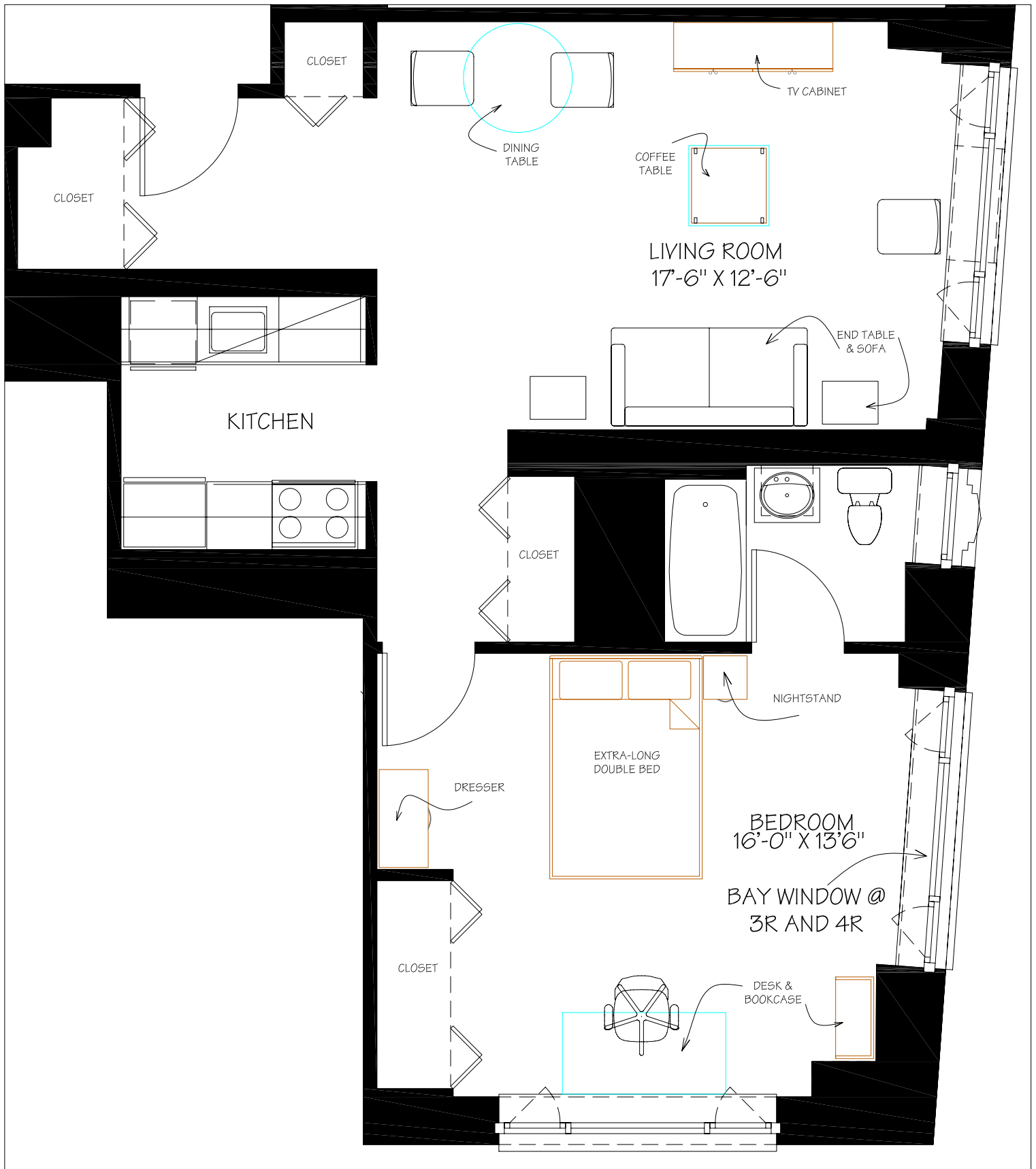
TYPE 7 Typical Apartment - 1 Bedroom - 650 sq.ft. Locations: 1Q and 2R - 5R 5apts. Total # Type 7 apts. 5apts.
